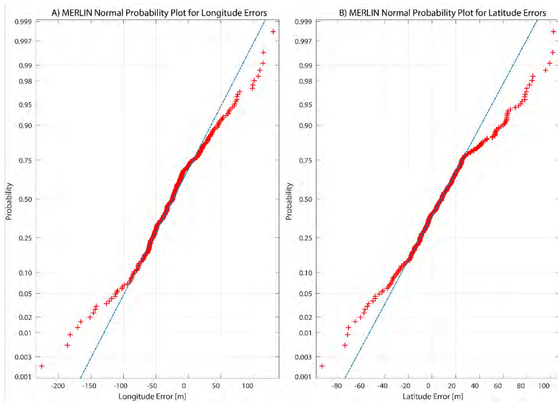
Fig 6. a) Normal probability plot for MERLIN longitude errors, and B) normal probability plot for MERLIN latitude errors.
